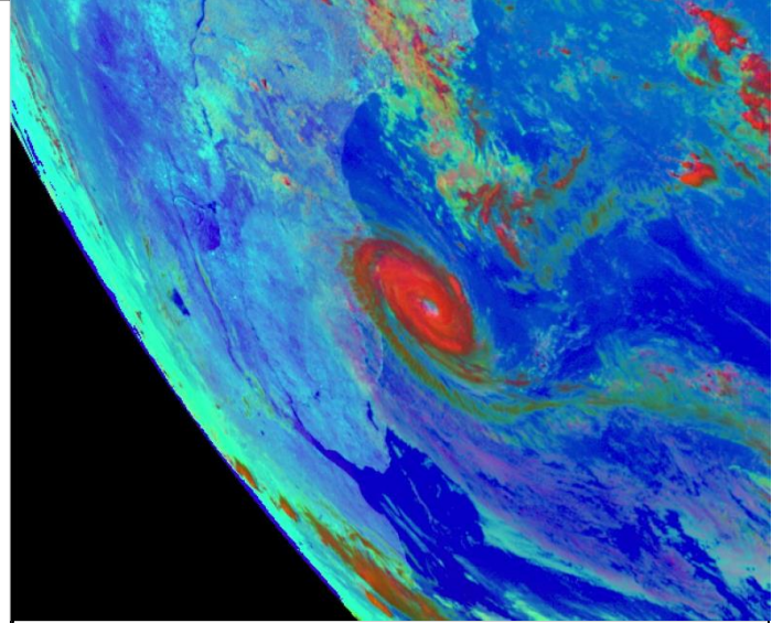
SEVIRI Day Micro RGB, 27 March 2004, 16:12 UTC
