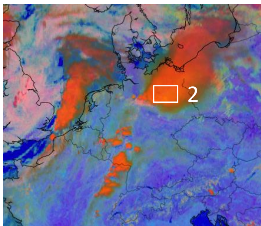
Day Microphysics RGB, 22 June 2017, 12:00 UTC
