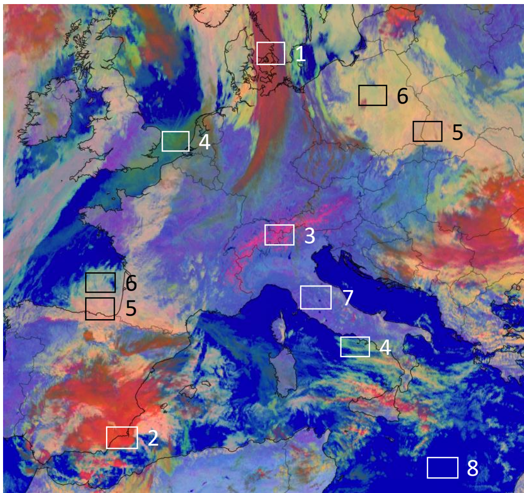
SEVIRI Day Microphysics RGB, 13 March 2017, 12:00 UTC
